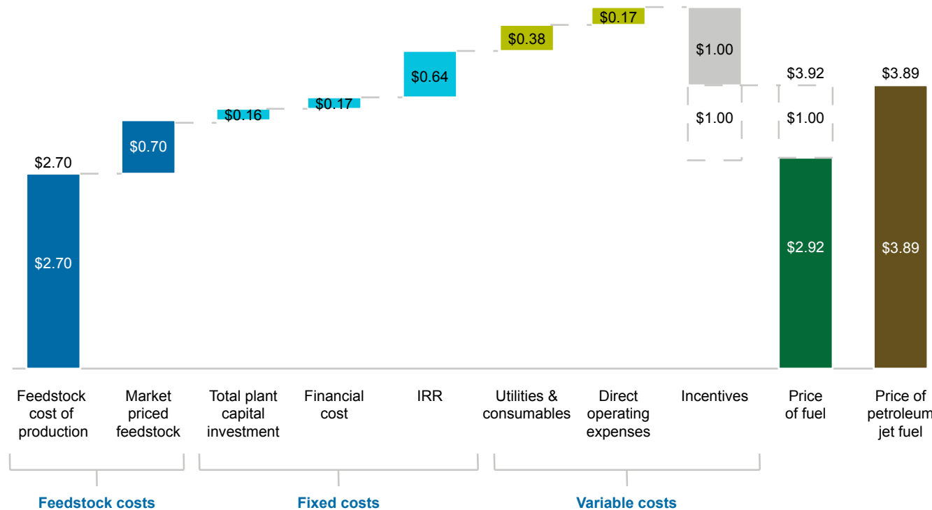
EXHIBIT 6: HEFA COST STRUCTURE
