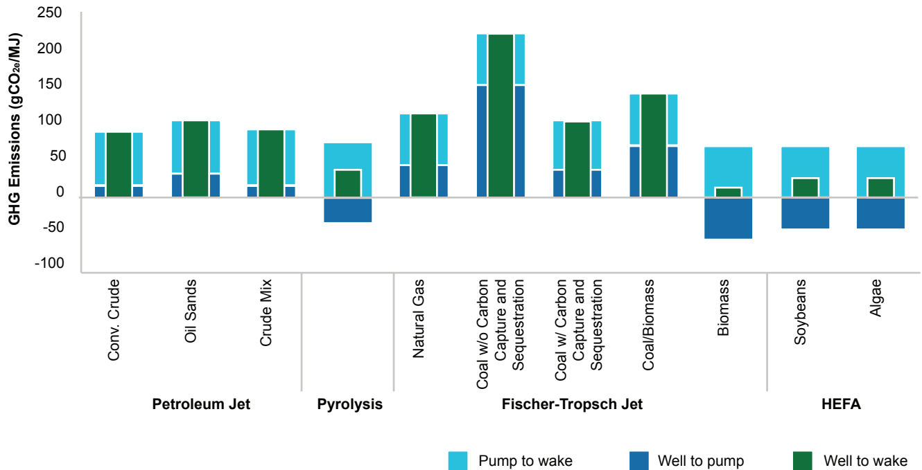
EXHIBIT 1: WELL TO WAKE GHG EMISSIONS BY ALTERNATIVE JET FUELS PRODUCTION PATHWAYS
