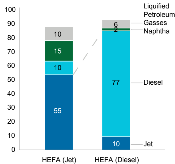
EXHIBIT 3: HEFA PRODUCT EFFICIENCY AND PRODUCT OUTPUT Output as a % of input weight
