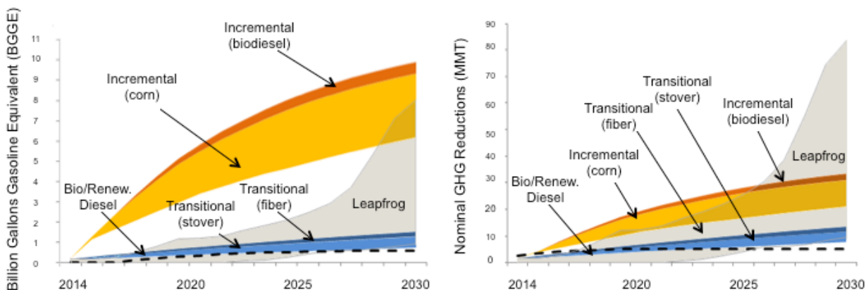
Figure 2: Maximum fuel production if specified route is aggressively pursued (left) and associated GHG reductions (right) in U.S.
