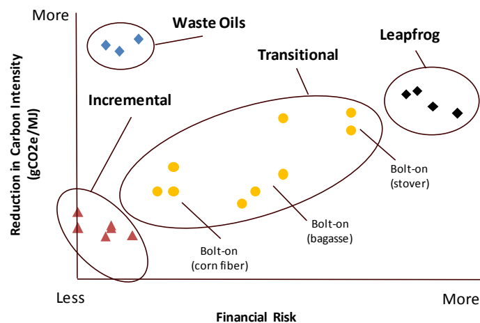
Figure 1: Conceptual graph of CO 2 e reduction potential and financial risk of biofuel pathway.
