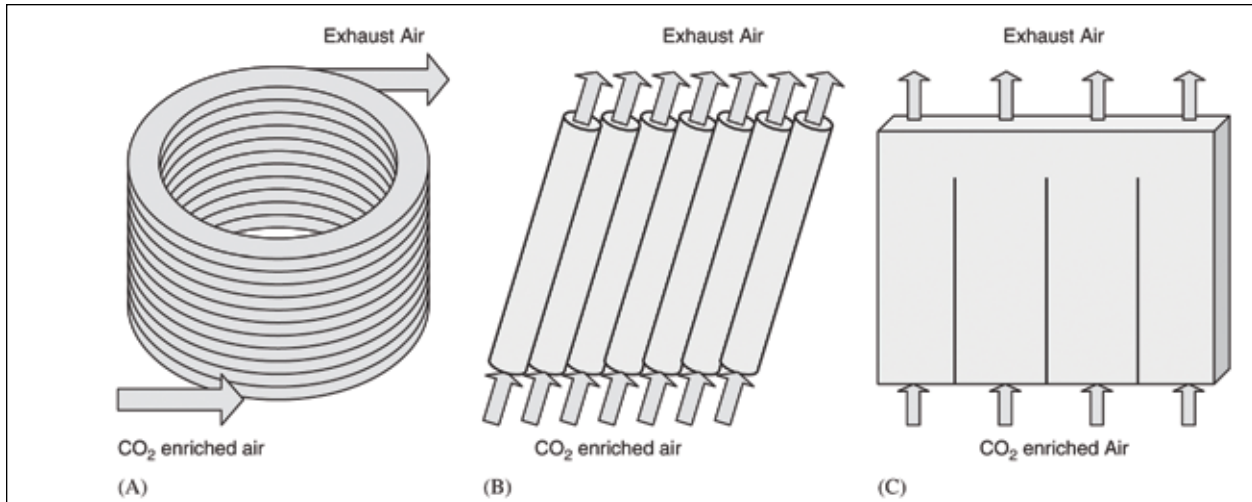
Figure 10: Some examples of translucent photobioreactors fed with air enriched with CO 2 for mass cultivation of algae. Source: Muñoz and Guieysse, 2006.
